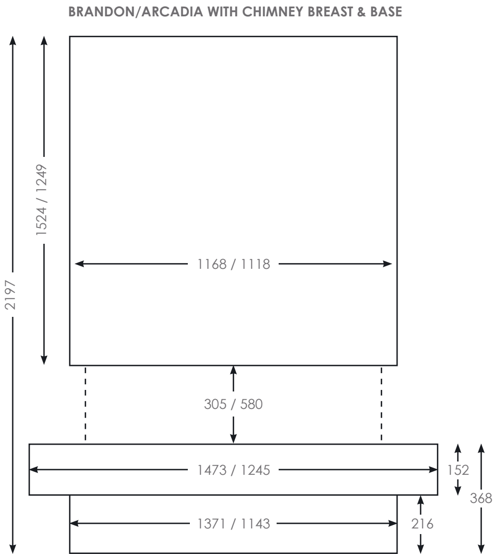
DEPTH: 355mm chimney breast & base / 410mm hearth
